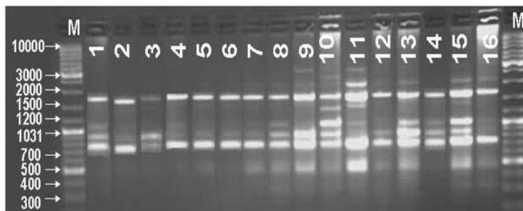
Figure 1. RAPD profile of 1–16 Cyamopsis tetragonoloba genotypes amplified with arbitrary primer OPA-16.
