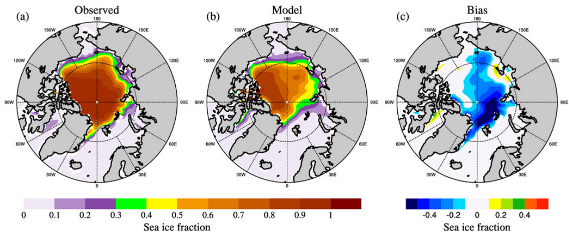
Figure S1: Same as figure 1, but with NSIDC observed data set
