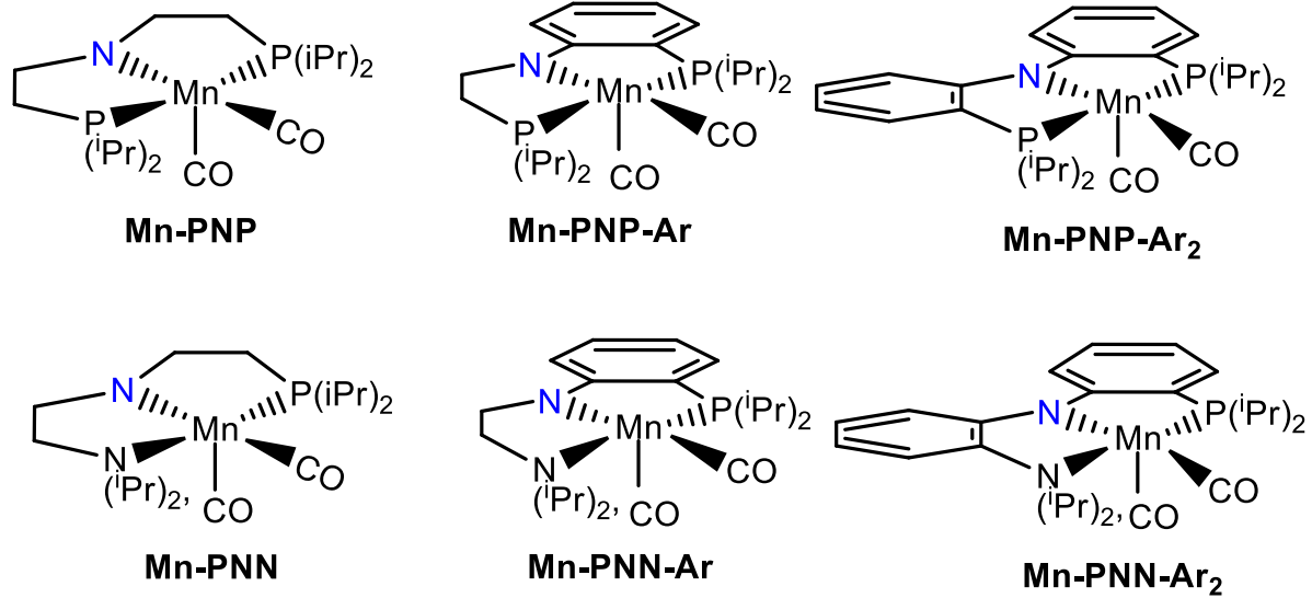
S1. Figure S1. Our modelled aliphatic amido Mn(I) pincer complexes for CO 2 hydrogenation reaction.
