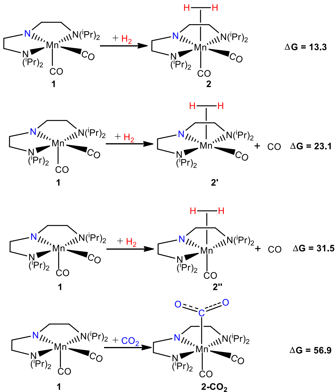
S2. Figure S2. The calculated reaction free energies ( \Delta G in kcal/mol) for the formation of different intermediates from 1 for Mn-NNN.
