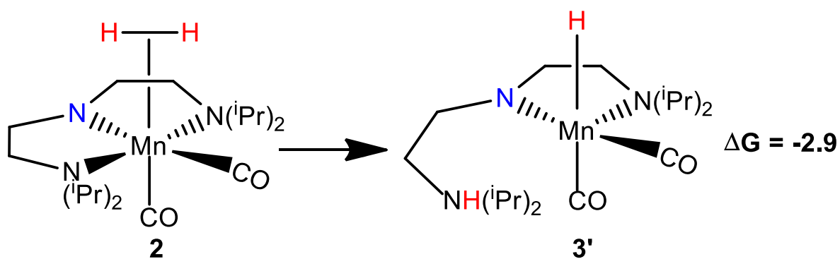
S2. Figure S3. The calculated reaction free energies ( \Delta G in kcal/mol) for heterolytic H 2 cleavage for Mn-NNN.
