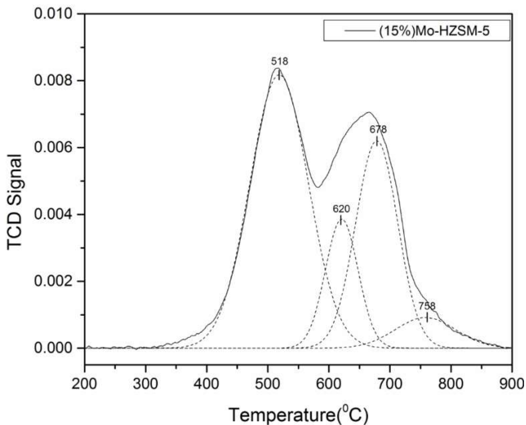
Figure S1. H 2 -TPR profile of 15%Mo-HZSM-5
