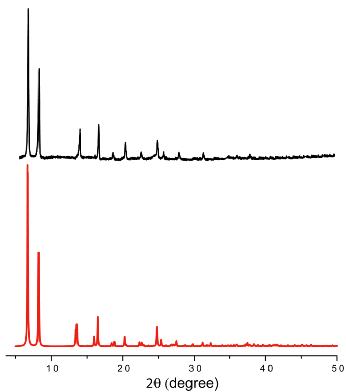
Figure S2. PXRD patterns of 1; red: simulated, black: as-synthesized.
