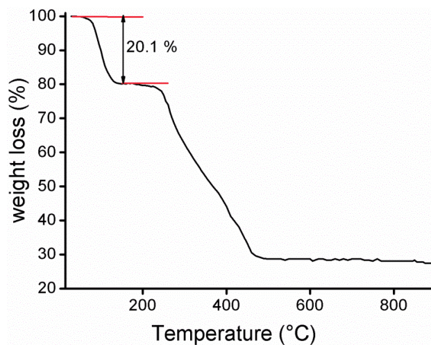
Figure S1. Thermogravimetric profile for complex 1.
