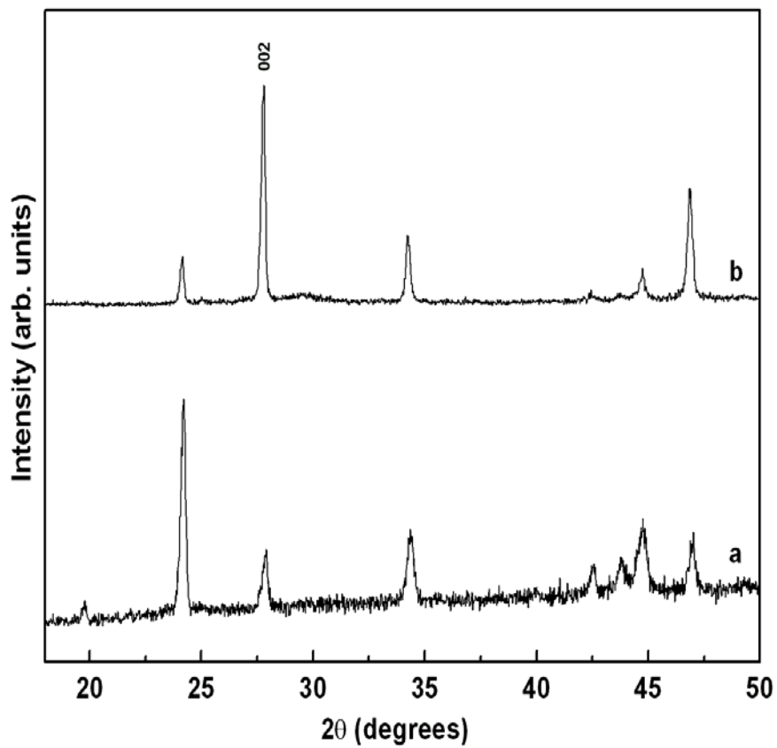
Figure S1. PXR D patterns of \text{BaCO}_3 coatings obtained from (a) DTPA-stabilized bath and (b) NTA-stabilized bath.
