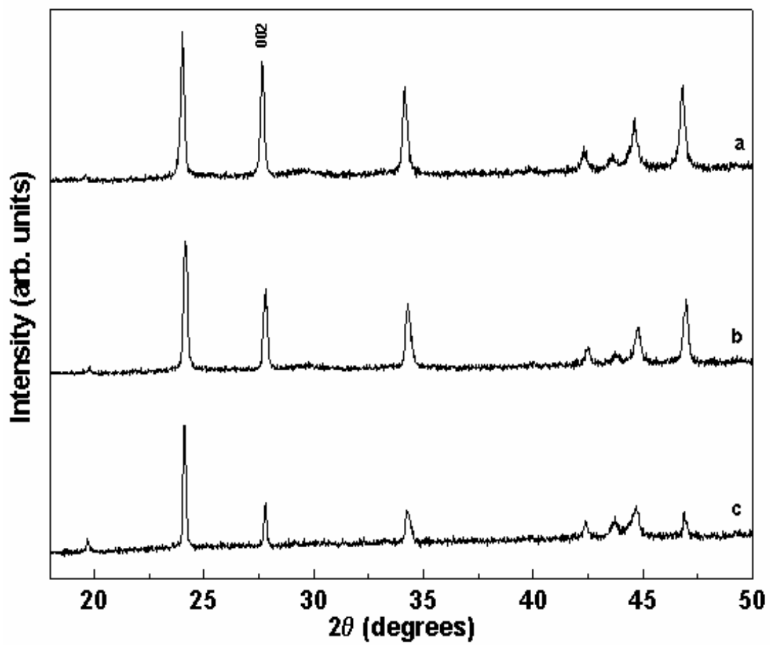
Figure S2. PXRD patterns of BaCO 3 coatings obtained from DTPA stabilized coatings at (a) pH 3.5 (b) 5.5 and (c) pH 7.0.
