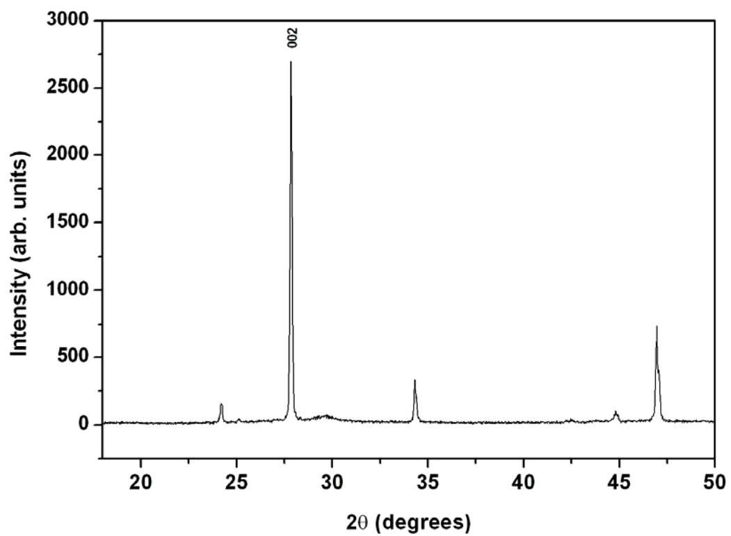
Figure S3. PXRD patterns of a BaCO 3 coating obtained from a DTPA stabilized bath at high current density.
