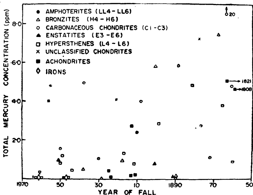
Figure 1. Total Hg concentrations of different classes of meteorites as a function of their year of fall. For meteorites with more than one measurement a mean value is taken; for Orgueil a mean value of 20 is indicated. See text and the footnotes of table 1 for further details.
