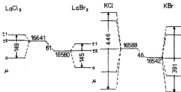
FIG. 2. ^1D_2 level of Pr^{3+} and its splittings in different crystals. Energy values are in cm^{-1} .
