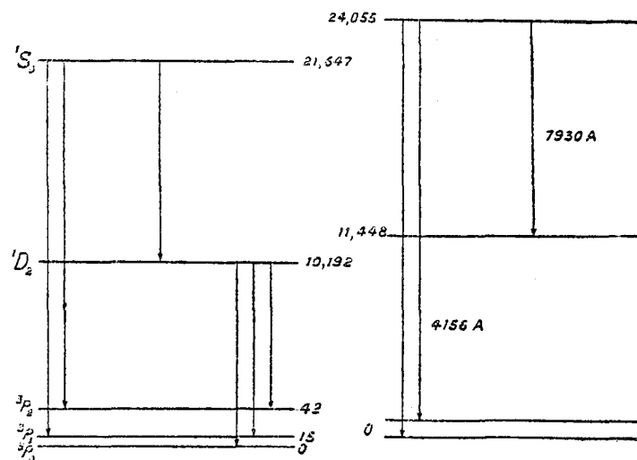
FIG. 1a. Energy levels in carbon atom
