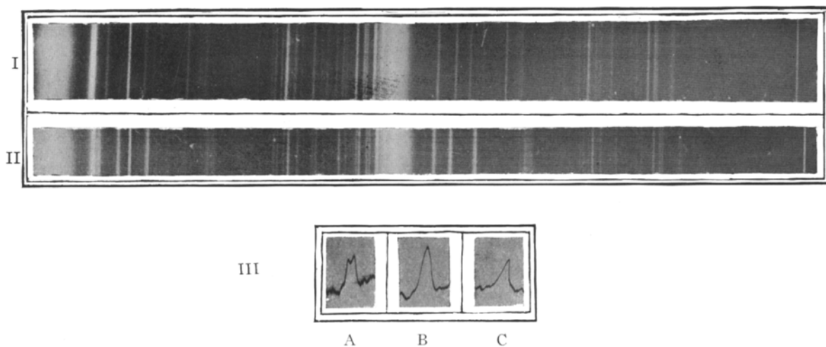
Fig. I. Coumarin in chloroform. Fig. II. Coumarin in carbon tetrachloride. Fig. III. Microphotometric records of the C = O frequency: (A) Solid, (B) Chloroform solution; (C) Carbon tetrachloride solution.
