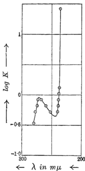
FIG. 5. (\text{C}_2\text{H}_5)_2\text{SO}_4 in substance.
