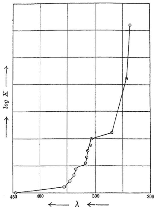
FIG. 6. \text{H}\cdot\text{Cl}\cdot\text{SO}_3 in substance.
