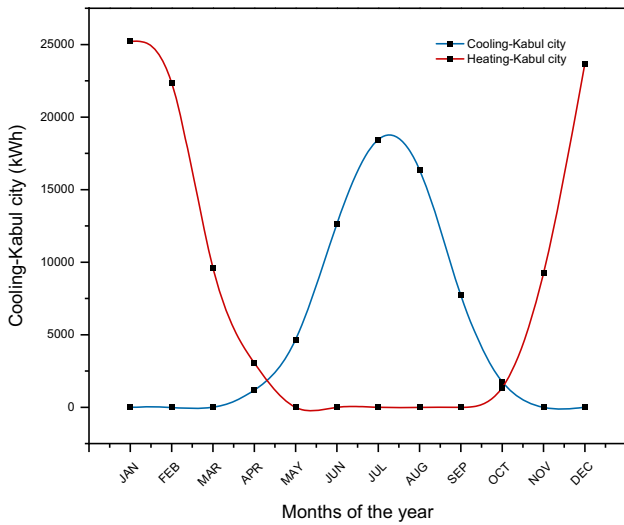
Figure 9. Base case-building annual energy consumption for Kabul city.
