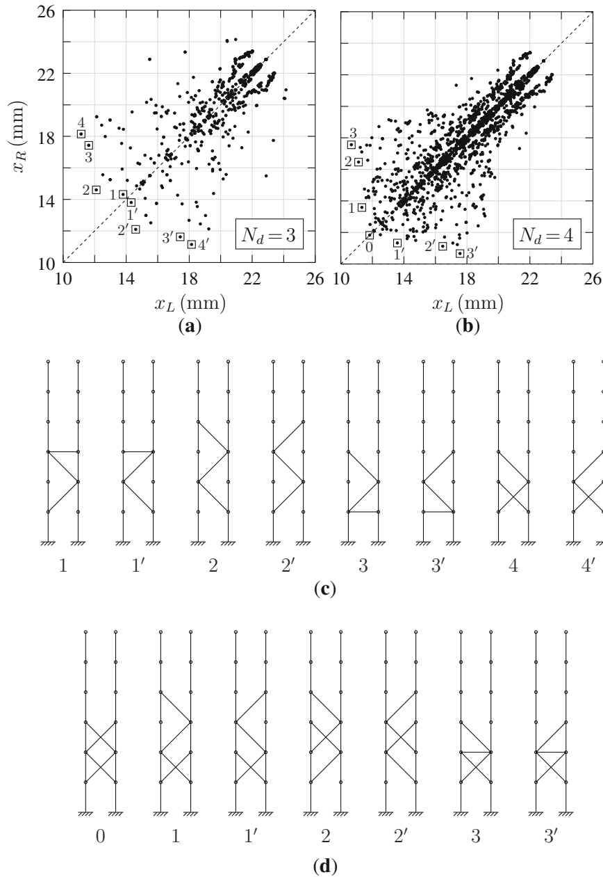
Figure 3. Maximum top left floor and top right floor displacements for six-storeyed DSABs: (a) solution space for N_d = 3 , (b) solution space for N_d = 4 , (c) damper placement for Pareto-optimal solutions with N_d = 3 and (d) damper placement for Pareto-optimal solutions with N_d = 4 .
