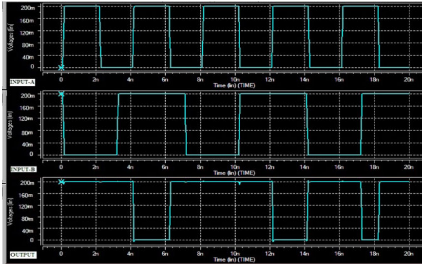
Figure 5. Transfer characteristics of 3T NAND gate @ 22 nm.
