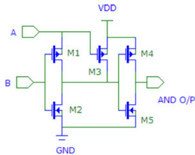
Figure 4. AND gate.
