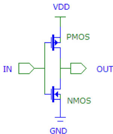
Figure 1. CMOS inverter.
