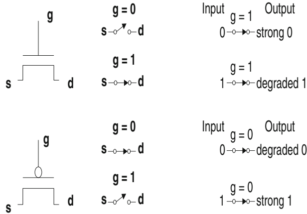
Figure 2. Pass transistor logic.
