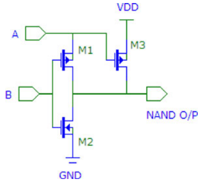
Figure 3. 3T NAND.
