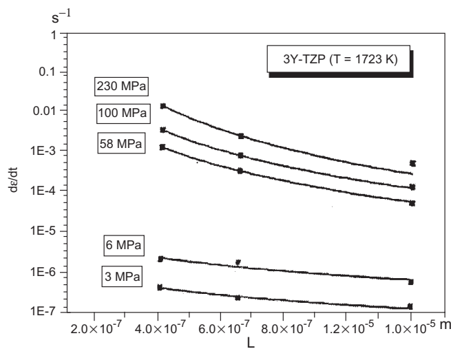
Figure 8. Log strain rate versus grain size plots according to (11) in ZrO_2-3\text{ mol}\% Y_2O_3 (3Y-TZP) polycrystalline material.
