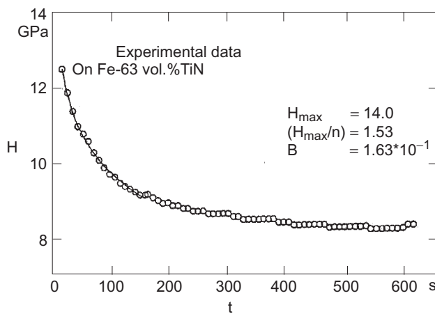
Figure 6. Hardness variation with time in Fe-63 vol% TiN which obeys (15).
