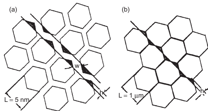
Figure 3. 2D schematic for plane interface formation in (a) nano ( W/L = 01 , L = 5 \text{ nm} ) and (b) micrometre ( W/L = 0005 , L = 1 \mu\text{m} ) grained materials. Atoms in the darker regions have to be rearranged by local boundary migration.
