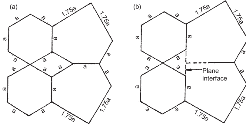
Figure 4. Schematic to show that plane interface formation decreases boundary area in the direction of sliding but increases grain boundary area perpendicular to that direction. (a) Prior to and (b) after deformation.
