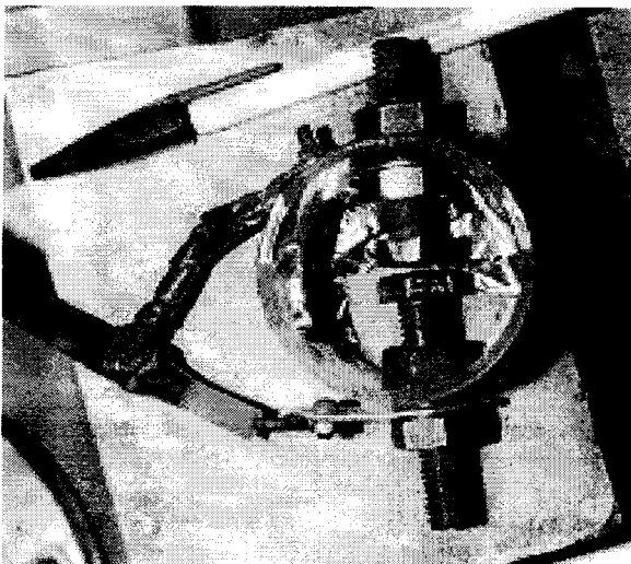
Figure 5. Spark gap switch.
