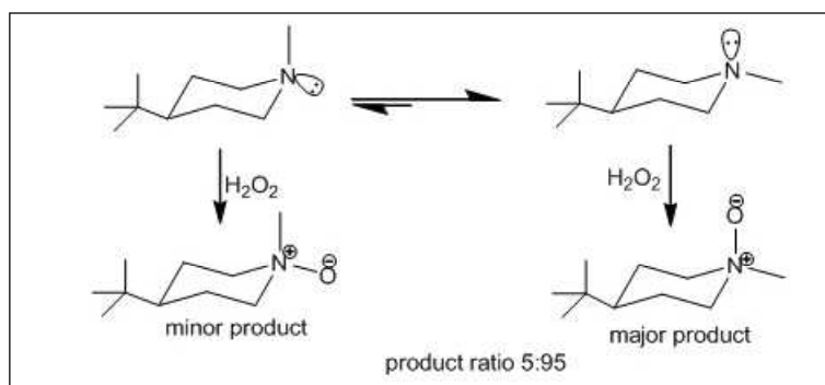
Scheme 7. Oxidation of 4- t -butyl- N -methylpiperidine.
