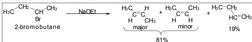
Scheme 2. Dehydrohalogenation of 2-bromobutane.
