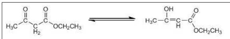
Scheme 9. Two tautomeric forms of ethyl acetoacetate (EAA).
