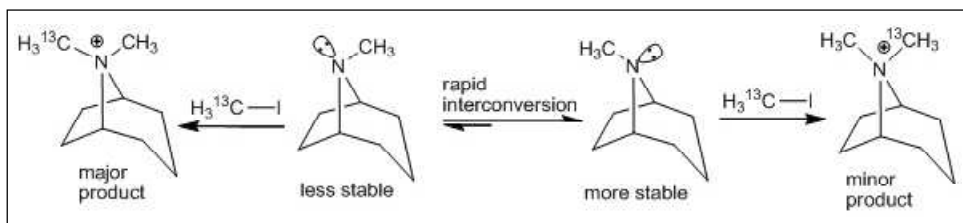
Scheme 5. Methylation of tropane.
