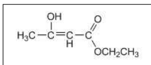
Figure 5. \beta -hydroxycrotonic ester.
