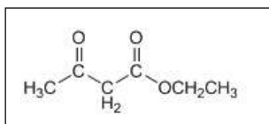
Figure 6. \beta -ketobutyric ester.
