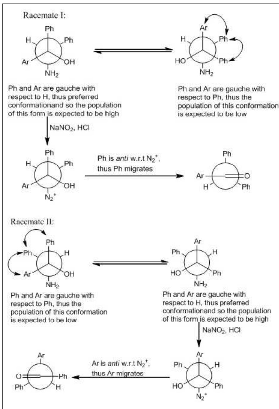
Scheme 14. Rearrangement of aminoalcohols.
