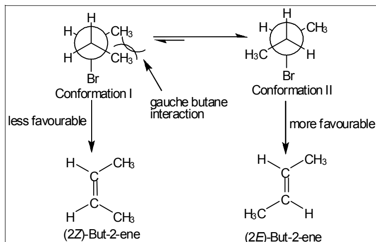
Scheme 3. Conformational analyses to obtain two isomeric 2-butenes.
