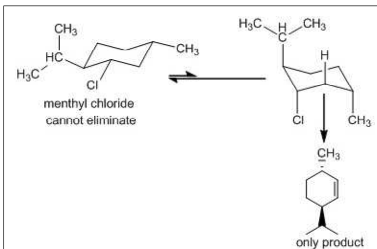
Scheme 6. Elimination of menthyl chloride under alkaline condition.
