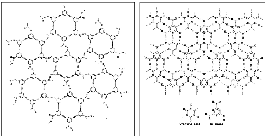
Figure 7 (top left). Rigid 'washers' held together by hydrogen bonds in a two-dimensional sheet.
