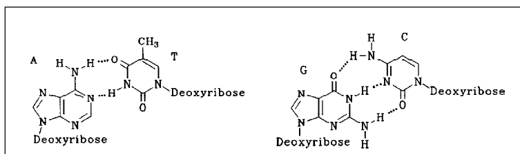
Figure 5. Hydrogen-bond directed mutual recognition of Adenine-Thymine (left) and Guanine-Cytosine (right).
