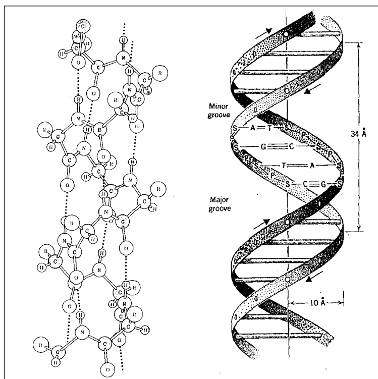
Figure 3 (left). An \alpha -helix. Note the N-H \cdots O hydrogen bonds parallel to the helix axis.
