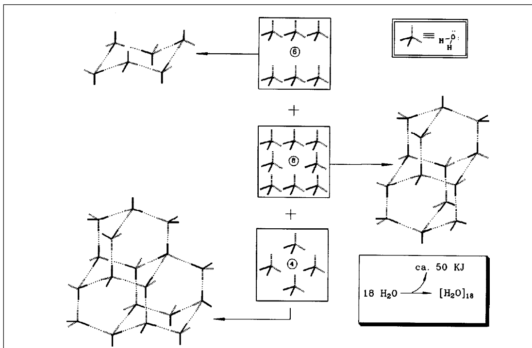
Figure 2. Assembly of water molecules in diamondoids.
