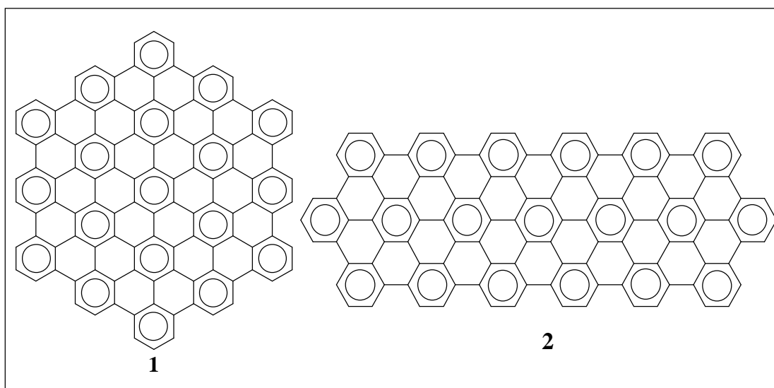
Figure 1. Two large graphenes, both with 114 carbon atoms: 1 = C_{114}H_{30} ; 2 = C_{114}H_{34} .
