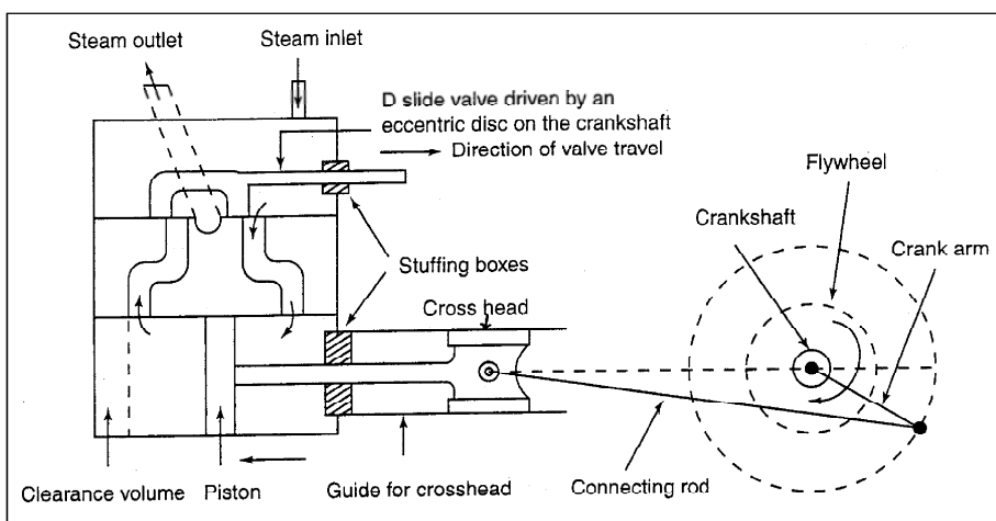
Figure 1. The Double-acting Steam Engine
