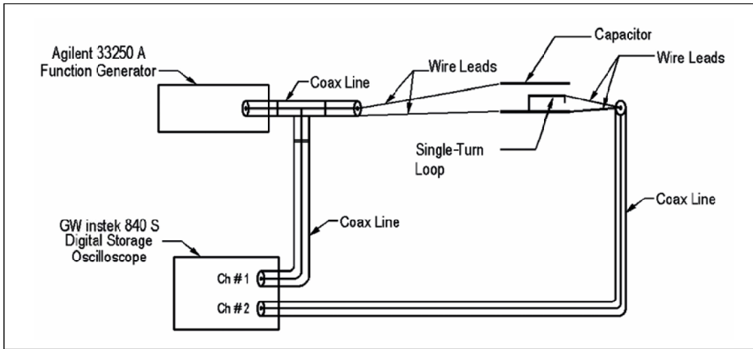
Figure 2. Schematic experimental setup for measurement of V_1 and V_2 described in the text.
