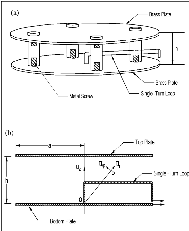
Figure 1. (a) Isometric view of the parallel plate air capacitor. (b) Schematic diagram of the capacitor showing the single-turn loop.
