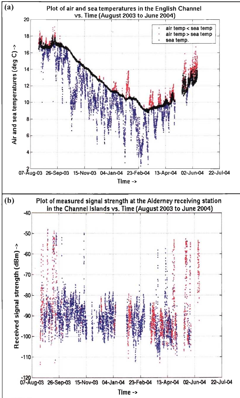
Figure 4. (a) The variation in the air and sea temperatures in the English Channel with time (from August 2003 to June 2004) (blue data = times when T_{air} < T_{sea} ; red data = times when T_{air} > T_{sea} ). (b) The signal strength measured at the Alderney receiving station antenna in the Channel Islands as a function of time (blue data=times when T_{air} < T_{sea} ; red data = times when T_{air} > T_{sea} .)
