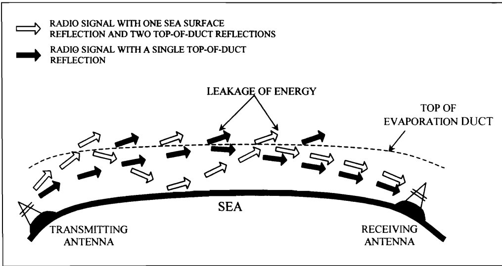
Figure 3. Diagram illustrating evaporation duct propagation.
