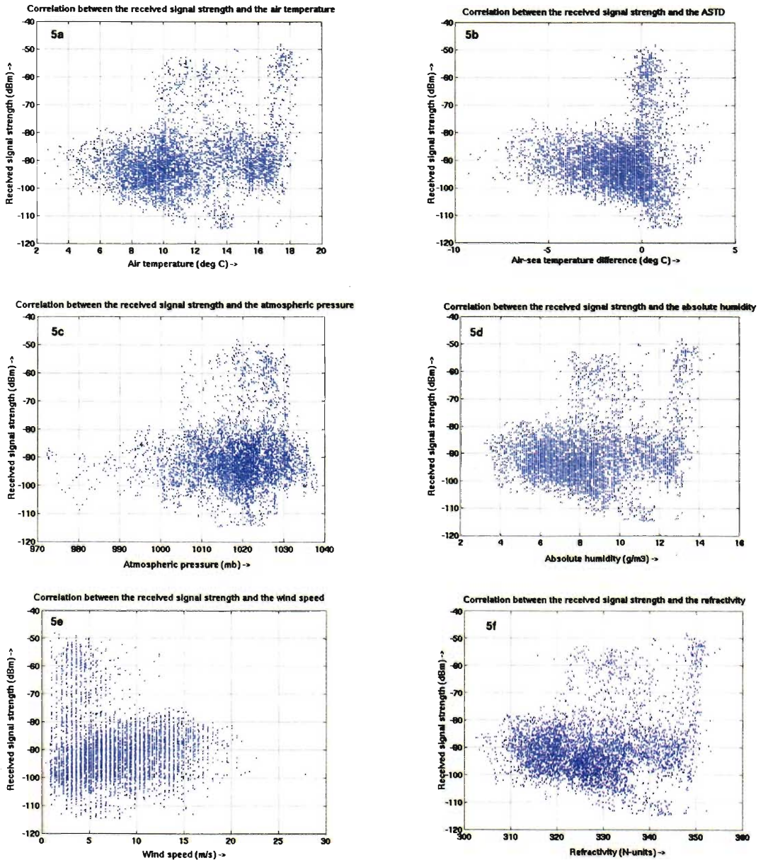
Figure 5. Graphs illustrating the correlation between the measured signal strength at the Alderney receiving station antenna in the Channel Islands and the various marine meteorological parameters time (from August 2003 to June 2004)
