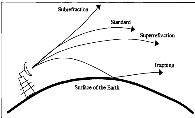
Figure 1. Diagram illustrating the four refractive conditions in the troposphere.
