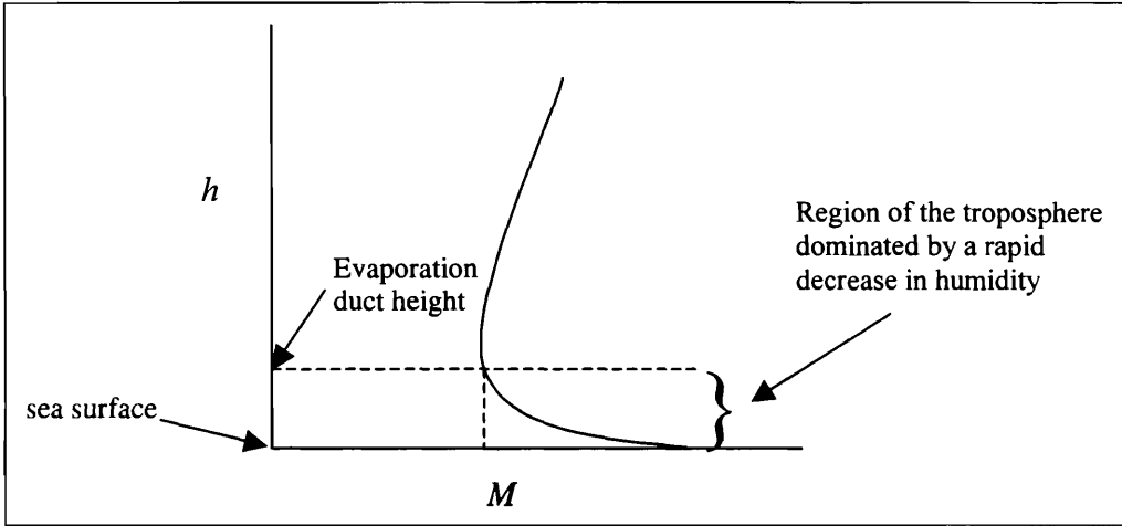
Figure 2. Modified refractivity profile of the troposphere above the surface of the sea indicating the presence of an evaporation duct.
