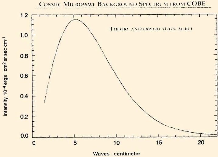
Figure 1. The blackbody fit to the spectrum of the CMB.
