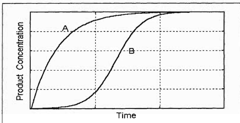
Figure 1. Curve A will be observed if the steps are just normal first order steps. Curve B is typical of an autocatalytic reaction.
