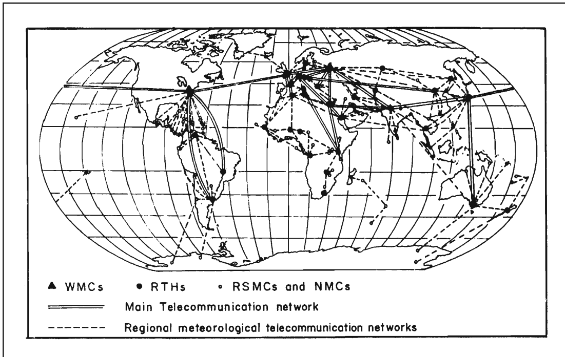
Figure 3 The Global Teleconnection System (GTS) (Adopted from WMO Bulletin , Vol. 45, January 1996).
