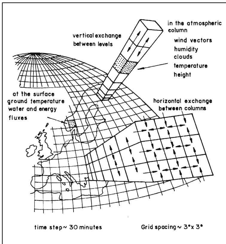
Figure 1 A cartesian grid for solving the meteorological equations .
