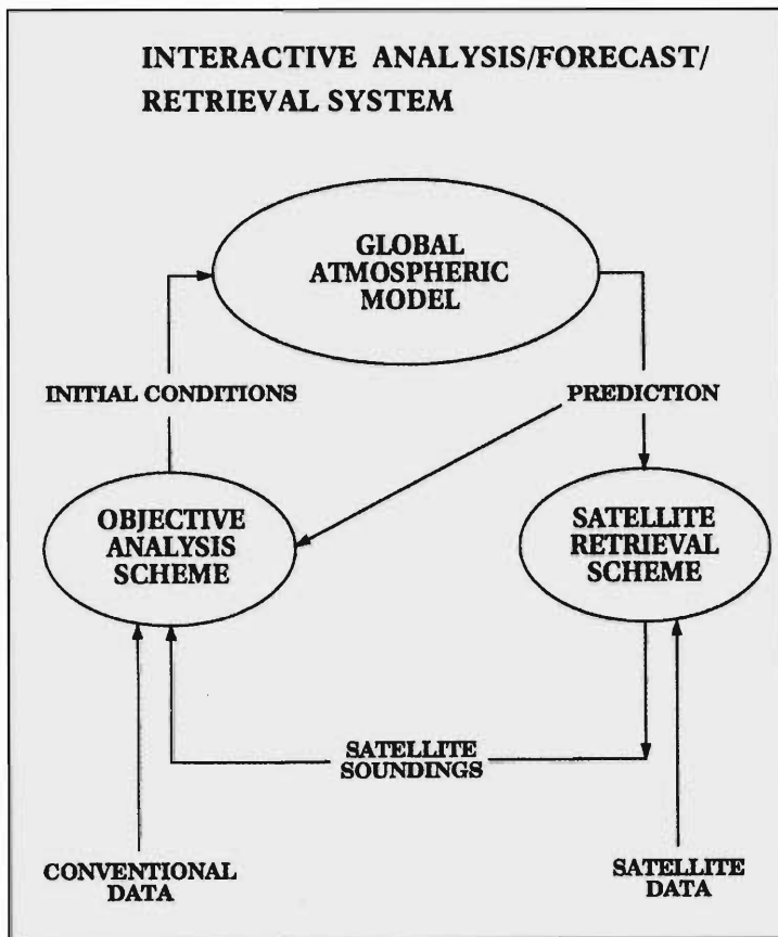
Figure 4 Schematic diagram of an interactive analysis/forecast/retrieval system.
