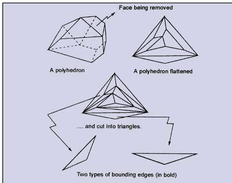
Figure 1 Euler's proof
