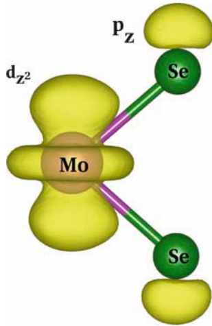
Figure 5. The charge density plot for the monolayer MoSe 2 for the highest occupied band at \Gamma point obtained from ab-initio calculations using GGA potentials at 0% strain.
