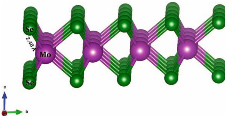
Figure 2. Crystal structure of a monolayer of MoSe 2 .
