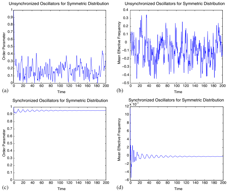
Figure 1. Unsyncronized and synchronized states of oscillators for symmetric natural frequency distribution. (a) shows the variation of coherence parameter with time and (b) shows the corresponding mean frequency variation for an unsynchronized state. (c) and (d) show the counterparts for a synchronized state.
