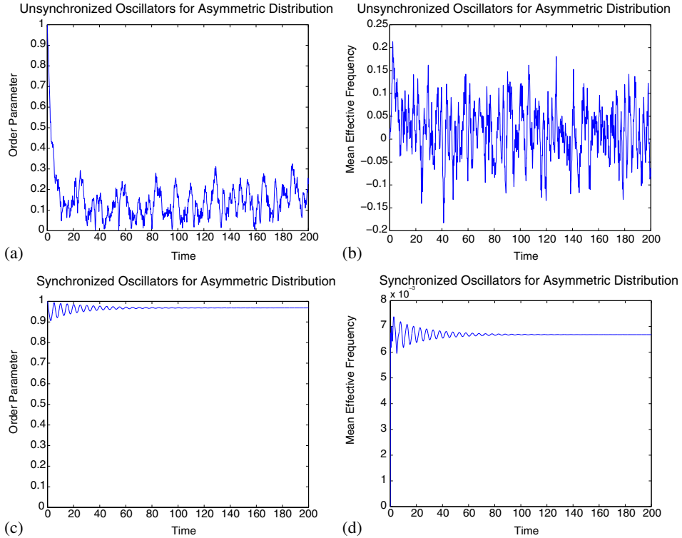
Figure 2. Unsynchronized and synchronized states of oscillators for asymmetric natural frequency distribution. (a) shows the variation of coherence parameter with time and (b) shows the corresponding mean frequency variation for an unsynchronized state. (c) and (d) show the counterparts for a synchronized state.
