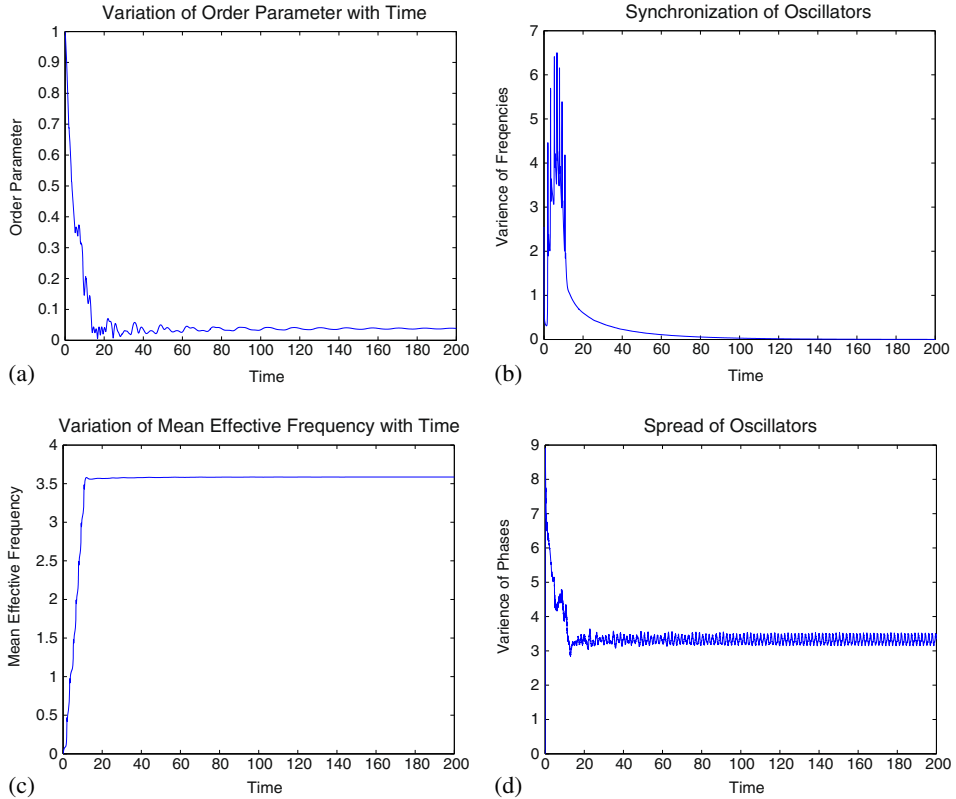
Figure 3. Numerical results of simulations with asymmetric distribution of natural frequencies. The network gets synchronized as seen by the variance of frequency decaying down to zero (in (b) ). For the same simulation, the coherence parameter (in (a) ) attains a very low value and the mean effective frequency (in (c) ) – which is the common synchronization frequency for asymptotically low variance – settles to a value away from the mean of the natural frequencies. (d) shows the variance of the phases which stabilizes to a finite value showing the spread of oscillators in the synchronized state.
