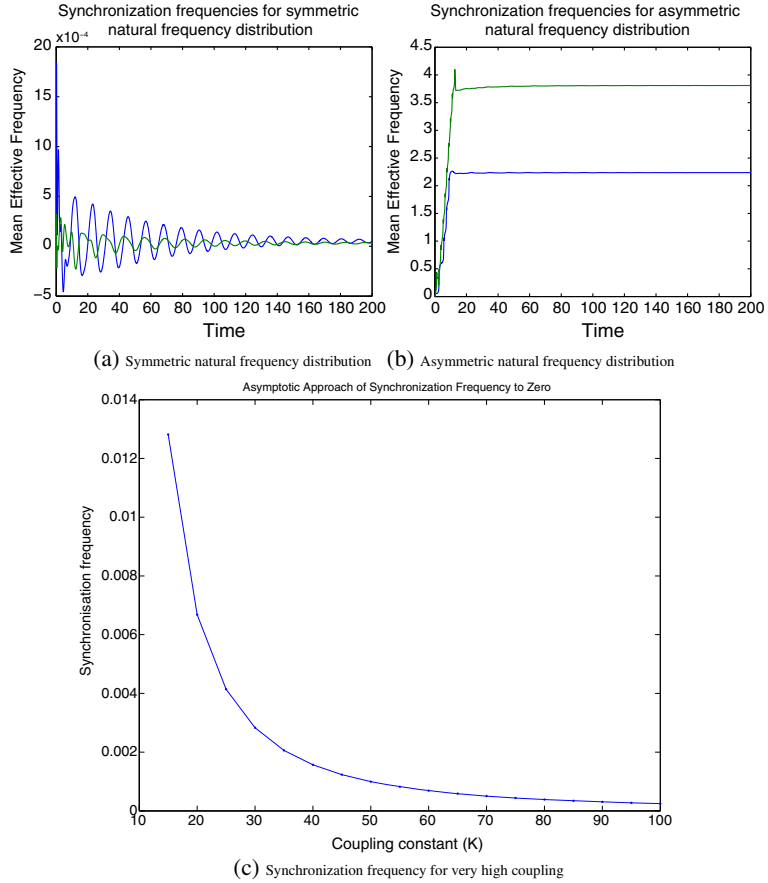
Figure 4. Effect of coupling strength on synchronization frequency. (a) and (b) show the time evolution of mean frequency for K = 8 (green) and K = 9 (blue) for symmetric and asymmetric natural frequency distributions. Synchronization occurs in both the cases. However, the synchronization frequency is unaffected (remains at zero) for the symmetric case, whereas it changes for its counterpart. As shown in (c), the synchronization frequency reaches zero for very high coupling strength.
