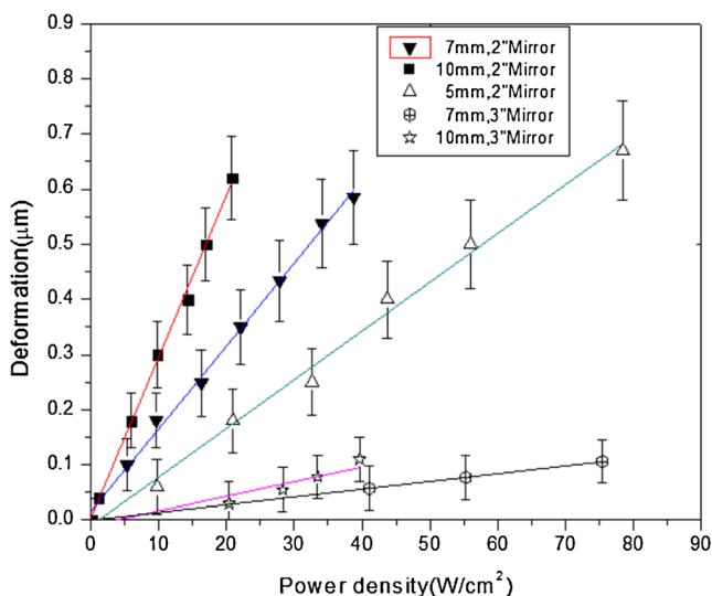
Figure 4. Deformation vs. average power density for mirrors with BK7 substrate. The inset data show spot size and mirror diameter.
