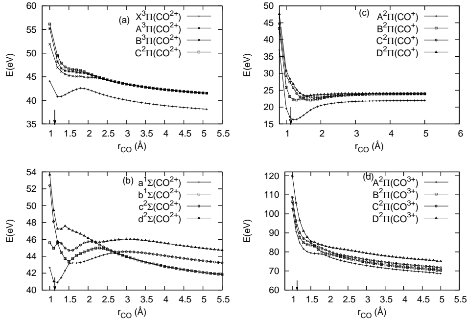
Figure 2. PECs for some of the excited states of CO + , CO 2+ , CO 3+ as obtained from MRCI/CASSCF calculations. The arrow along the x -axis in panels (a–d) shows the value of r_e for the ground state of neutral CO.
