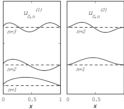
Figure 3. Eigenfunctions for supersystems with l = 0 . Corresponding eigenenergies are shown by dashed lines.
