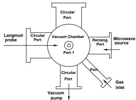
Figure 3. Main chamber (axial view).
