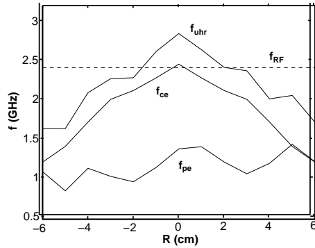
Figure 13. Radial variation of f_{ce} , f_{pe} and f_{uhr} .
