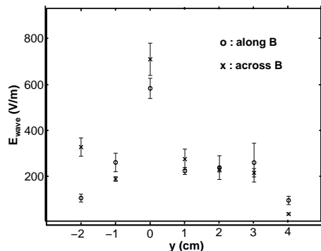
Figure 16. Electric field of the outgoing EM wave.
