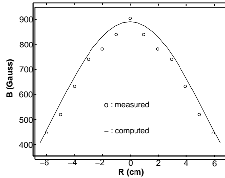
Figure 5. Radial variation of the magnetic field in the system.
