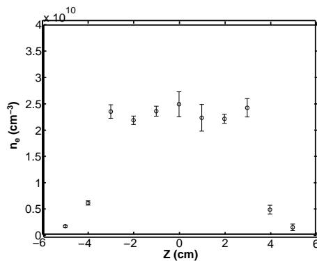
Figure 8. Axial variation of plasma density.
