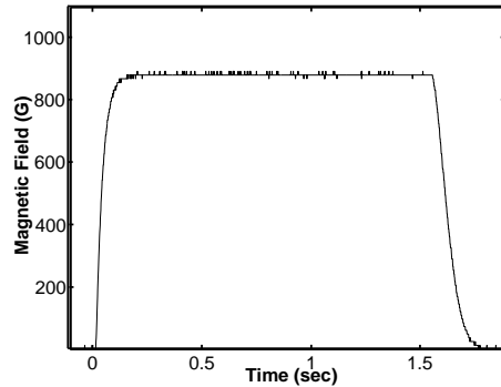
Figure 7. Time evolution of magnetic field.
