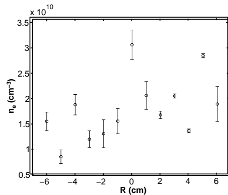
Figure 9. Radial variation of plasma density.
