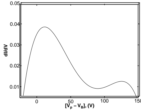
Figure 15. EEDF at the centre of the system.
