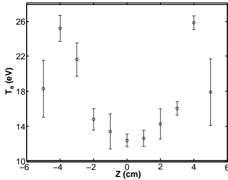
Figure 10. Axial variation of plasma temperature.
