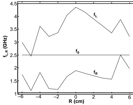
Figure 14. Radial variation of \omega_L and \omega_R .
