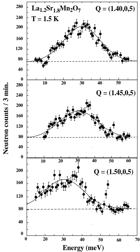
Figure 8. Energy scans at T = 1.5 K close to the zone boundary corresponding to Q = (1.40, 0, 5) , (1.45, 0, 5) , and (1.50, 0, 5) .
