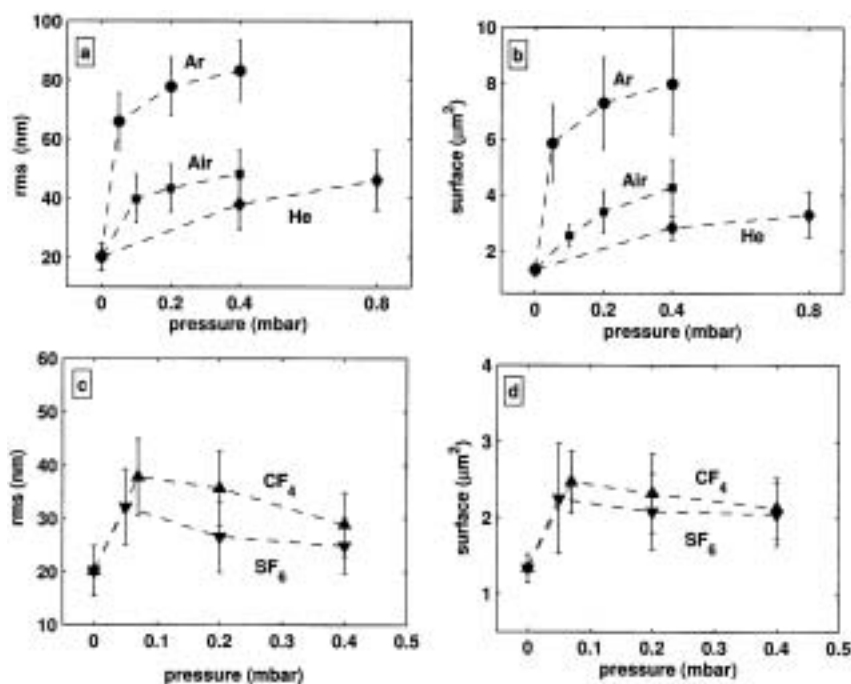
Figure 7. Rms surface roughness and surface area of plasma treated PET fabrics as a function of the plasma gas pressure using different gases: (a) rms surface roughness of air, He and Ar plasma gases, (b) surface area for air, He and Ar plasma gases, (c) rms surface roughness for SF 6 and CF 4 plasma gas, (d) surface area for SF 6 and CF 4 plasma gas.
