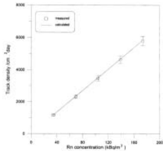
Figure 5. Comparison between measured and calculated LR-115 efficiency.
