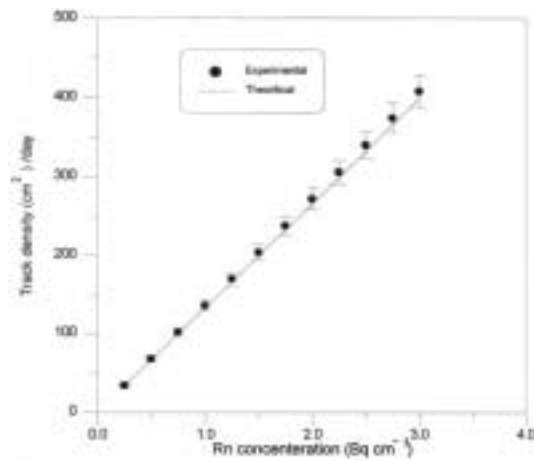
Figure 4. Comparison between measured and calculated CR-39 efficiency.
