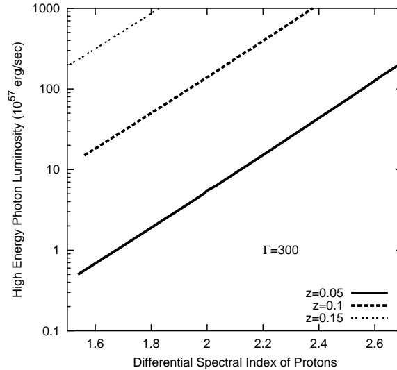
Figure 1. The minimum luminosity in the high-energy component required for detection with a signal-to-noise ratio of 5 or larger in an ICECUBE class detector, as a function of the power-law index ( \alpha_p ) of the differential spectrum of protons accelerated within a typical GRB source, for various values of the red-shift z of the GRB. The values taken for other relevant parameters are as given in ref. [9].
