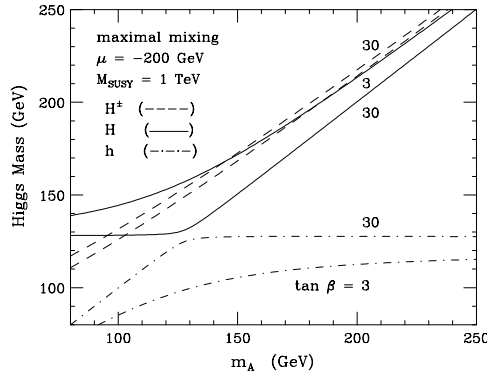
Figure 4. Higgs masses as a function of m_A for maximal mixing with m_{\text{SUSY}} = M_Q = M_U = M_D = 1 \text{ TeV} .
