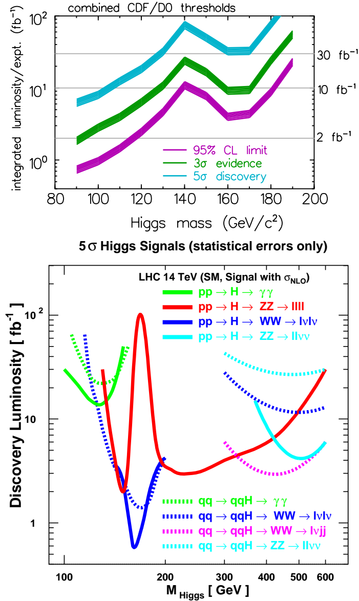
Figure 3. SM Higgs discovery at Tevatron and LHC. h_{SM} detection is guaranteed at the LHC.
