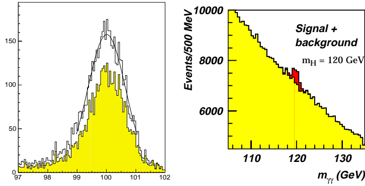
Figure 6. CMS simulations of background subtracted signal, including the recovered photon conversions (left, M_H = 100 GeV) and signal+background (right, M_H = 120 GeV) for the standard model Higgs decay to two photons are plotted vs. the reconstructed diphoton invariant mass.
