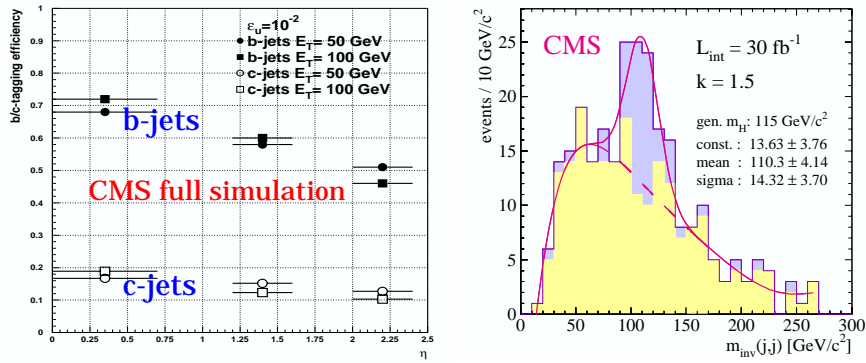
Figure 7. CMS detector b jet tagging efficiency (left) and signal for pp \rightarrow t\bar{t}H(\rightarrow b\bar{b}) (right) are shown.
