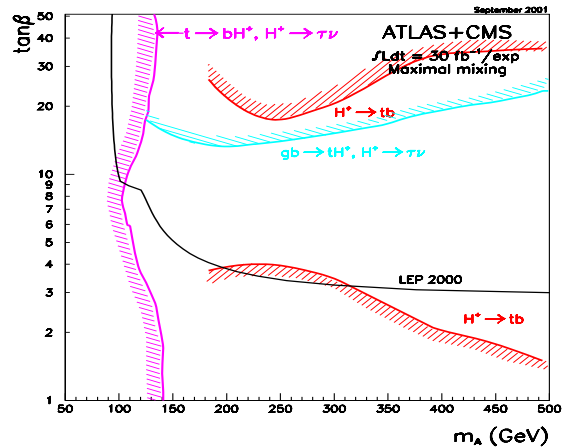
Figure 17. The summary of coverage of MSSM parameter space for charged Higgs decay is shown.
