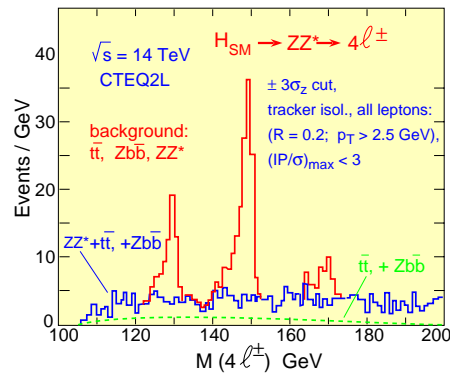
Figure 10. CMS simulation of Higgs decays to ZZ^* . M_H = 130, 150, 170 GeV is shown for the case where both the Z bosons decay into leptons.
