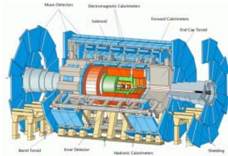
Figure 2. The ATLAS detector showing its subsystems.
