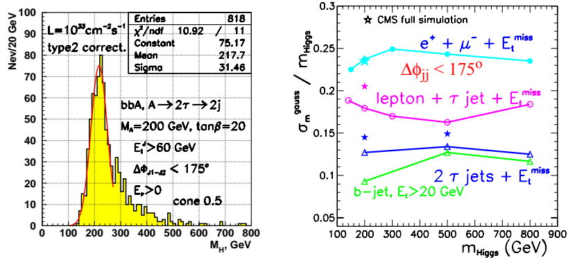
Figure 13. MSSM heavy Higgs mass peak (left) for its decay to \tau jet pairs is shown ( M_H = 200 GeV). Mass resolutions (right) for leptonic and hadronic decays of \tau are shown as a function of M_H .
