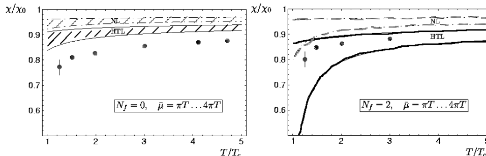
Figure 5. Comparison of lattice results with resummed, HTL and NL, perturbation theory for quenched QCD (left) and full QCD (right).
