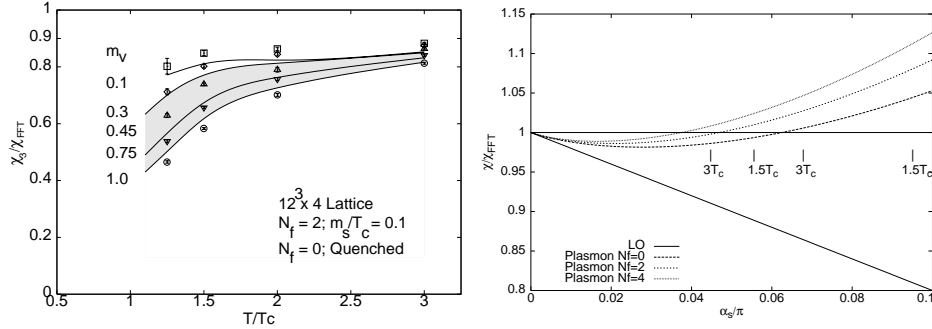
Figure 4. Quark number susceptibility from numerical simulations (left) and perturbation theory (right).
