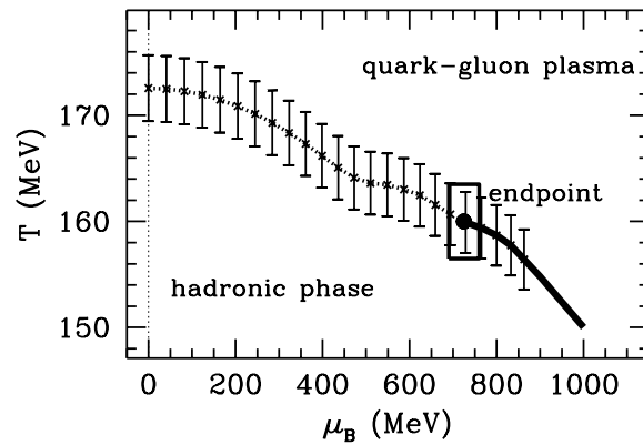
Figure 3. \mu_B - T phase diagram for QCD.
