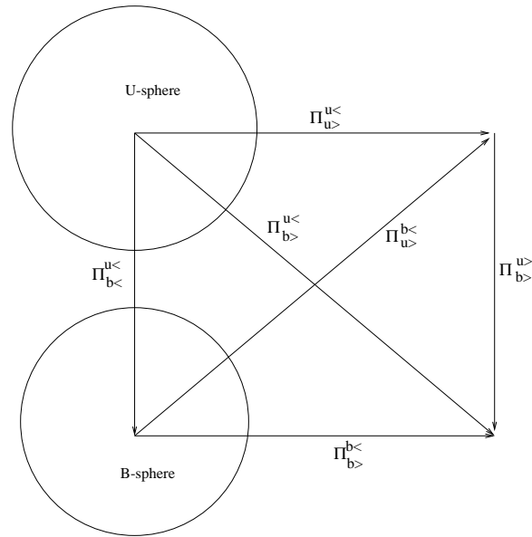
Figure 1. Various energy cascade rates of MHD turbulence. The illustrated wave-number spheres contain \mathbf{u} < and \mathbf{b} < modes, while \mathbf{u} > and \mathbf{b} > are modes outside these spheres. The velocity field is forced at large-scale.
