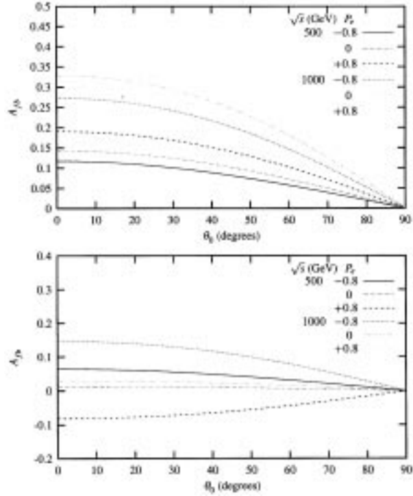
Figure 3. The asymmetry A_{fb} defined in the text, for Imc_d^\gamma = 1, Imc_d^Z = 0 (top), and for Imc_d^\gamma = 0, Imc_d^Z = 1 (bottom), plotted as a function of the cut-off \theta_0 on the lepton polar angle in the forward and backward directions for e^- beam longitudinal polarizations P_e = -0.8, 0, +0.8 and for values of total cm energy \sqrt{s} = 500 GeV and \sqrt{s} = 1000 GeV.
