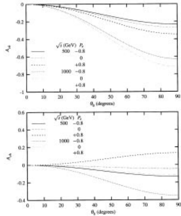
Figure 2. The asymmetry A_{ch} defined in the text, for Imc_d^\gamma = 1, Imc_d^Z = 0 (top), and for Imc_d^\gamma = 0, Imc_d^Z = 1 (bottom), plotted as a function of the cut-off \theta_0 on the lepton polar angle in the forward and backward directions for e^- beam longitudinal polarizations P_e = -0.8, 0, +0.8 and for values of total cm energy \sqrt{s} = 500 GeV and \sqrt{s} = 1000 GeV.
