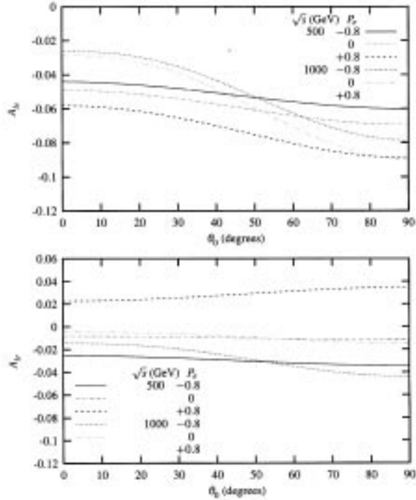
Figure 5. The asymmetry A_{lr} defined in the text, for \text{Im}c_d^\gamma = 0.1 , \text{Im}c_d^Z = 0 (top), and for \text{Im}c_d^\gamma = 0 , \text{Im}c_d^Z = 0.1 (bottom), plotted as a function of the cut-off \theta_0 on the lepton polar angle in the forward and backward directions for e^- beam longitudinal polarizations P_e = -0.8, 0, +0.8 and for values of total cm energy \sqrt{s} = 500 GeV and \sqrt{s} = 1000 GeV.
