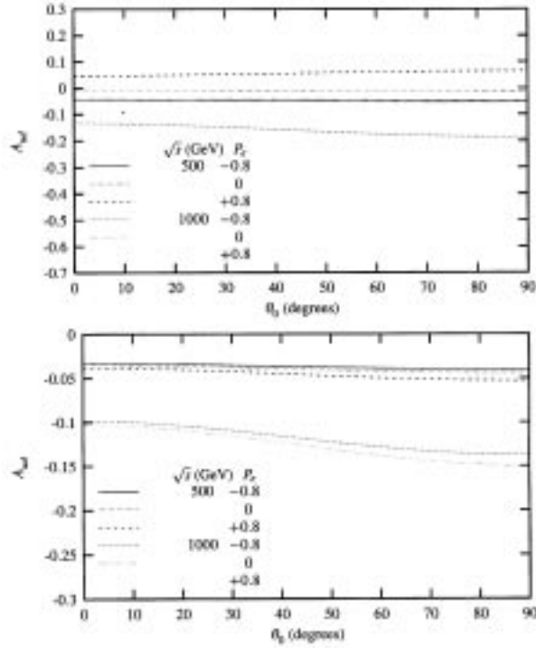
Figure 4. The asymmetry A_{ud} defined in the text, for Rec_d^\gamma = 0.1, Rec_d^\zeta = 0 (top), and for Rec_d^\gamma = 0, Rec_d^\zeta = 0.1 (bottom), plotted as a function of the cut-off \theta_0 on the lepton polar angle in the forward and backward directions for e^- beam longitudinal polarizations P_e = -0.8, 0, +0.8 and for values of total cm energy \sqrt{s} = 500 GeV and \sqrt{s} = 1000 GeV.
