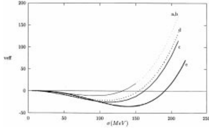
Figure 1. Effective potential in units of (100 \text{ MeV})^4 as a function of \sigma (MeV) for different values of the magnetic field. The curves a, b, c, d and e are for B = 0, 10^{16}, 10^{18}, 10^{19} and 3 \times 10^{19} G respectively.
