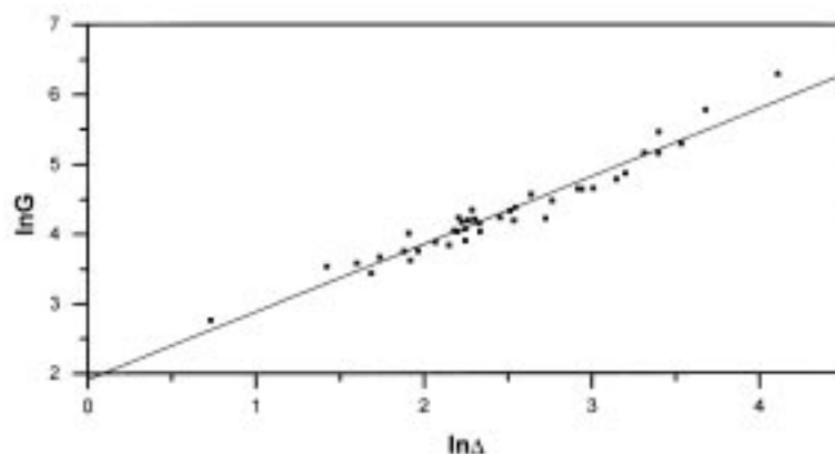
Figure 2. Graph of \ln G vs. \ln \Delta .
