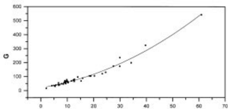
Figure 1. Graph of G vs. \Delta .
