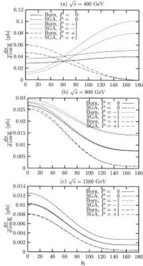
Figure 1. The distribution in \theta_l with and without QCD corrections for (a) \sqrt{s} = 400 GeV, (b) \sqrt{s} = 800 GeV and (c) \sqrt{s} = 1500 GeV plotted against \theta_l , for e^- beam polarizations P = 0, -1, +1 in each case.
