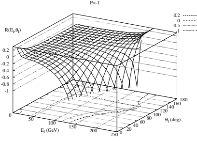
Figure 5. The ratio R(E_l, \theta_l) of the CP-violating part of the cross-section to the SM cross-section defined in the text for \text{Re}f_{2R} = -\text{Re}\bar{f}_{2L} = 10^{-2} with effective beam polarization P = -1 . A few contours of constant values of R are shown on the bottom plane.
