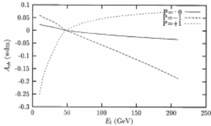
Figure 10. The charge asymmetry A_{\text{ch}} arising from the top weak dipole moment as a function of E_l for \theta_0 = 30^\circ for three values of the effective e^+e^- polarization P . The top wdm assumed is (0.1)e/m_t .
