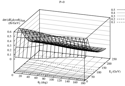
Figure 1. The standard model double differential cross-section as a function of energy E_l and polar angle \theta_l of the charged lepton l^+ (either \mu^+ or e^+ ) for unpolarized beams. The bottom plane shows a few contours of constant cross-section.
