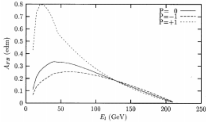
Figure 13. The asymmetry A_{FB} arising from the top electric dipole moment as a function of E_t for \theta_0 = 30^\circ for three values of the effective e^+e^- polarization P . The top edm assumed is e/m_t .
