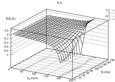
Figure 4. The ratio R(E_l, \theta_l) of the CP-violating part of the cross-section to the SM cross-section defined in the text for \text{Re}f_{2R} = -\text{Re}f_{2L} = 10^{-2} with unpolarized beams. A few contours of constant R values are shown on the bottom plane.
