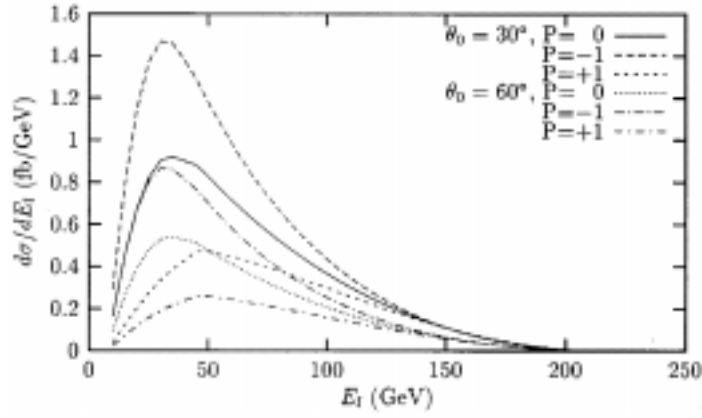
Figure 7. SM differential cross-section integrated over \theta_l with a cut-off \theta_0 in the forward and backward directions. The curves are shown for \theta_0 = 30^\circ and \theta_0 = 60^\circ and for effective beam polarizations P = 0, -1, +1 .
