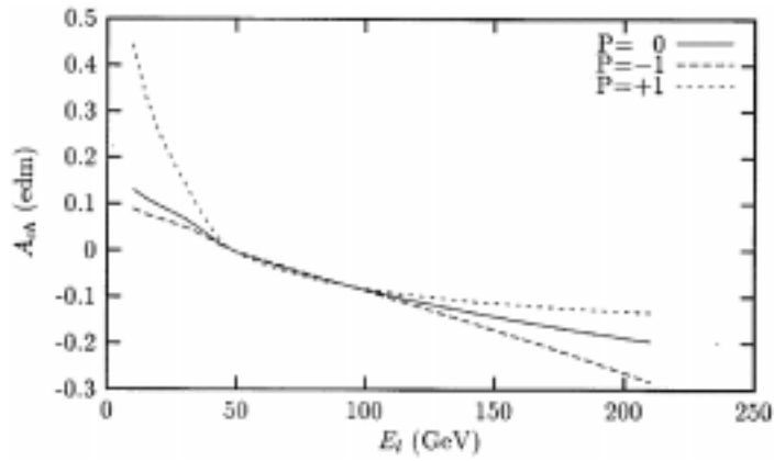
Figure 9. The charge asymmetry A_{\text{ch}} arising from the top edm as a function of E_l for \theta_0 = 30^\circ for three values of the effective e^+e^- polarization P . The top edm assumed is (0.1)e/m_t .
