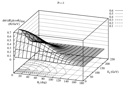
Figure 3. The standard model double differential cross-section as in figure 1, but for effective beam polarization P_{e^-} = -P_{e^+} = +1 . The bottom plane shows a few contours of constant cross-section.
