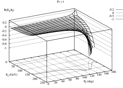
Figure 6. The ratio R(E_l, \theta_l) of the CP-violating part of the cross-section to the SM cross-section defined in the text for \text{Re}f_{2R} = -\text{Re}\bar{f}_{2L} = 10^{-2} with effective beam polarization P = +1 . A few contours of constant values of R are shown on the bottom plane.
