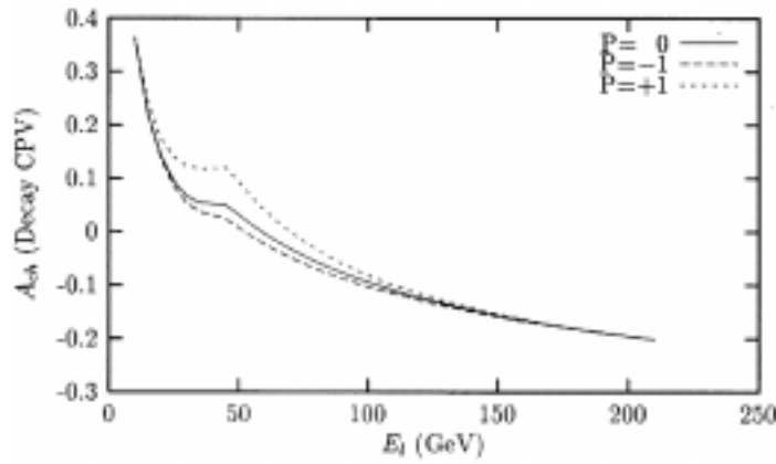
Figure 11. The charge asymmetry A_{ch} arising from the CP-violating tbW vertex as a function of E_l for \theta_0 = 30^\circ for three values of the effective e^+e^- polarization P . Re\bar{f}_{2R} = -Re\bar{f}_{2L} = 0.1 is assumed.
