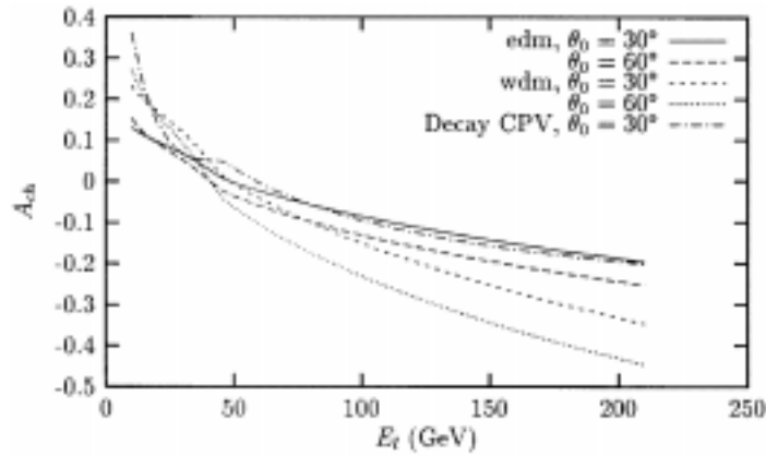
Figure 8. The charge asymmetry A_{ch} as function of E_l with two cut-off angles, for the different sources of CP-violation, and unpolarized beams. The top edm is taken to be (0.1)e/m_t , the wdm to be e/m_t , and Re f_{2R} = -Re f_{2L} = 0.1 .
