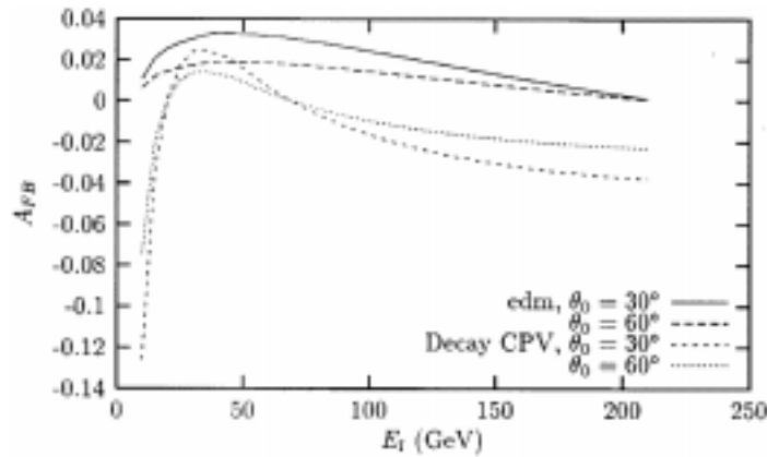
Figure 12. The asymmetry A_{FB} as function of E_l with two cut-off angles, for the different sources of CP-violation, for unpolarized beams. The top edm is taken as (0.1)e/m_t , and Re\bar{f}_{2R} = -Re\bar{f}_{2L} = 0.1 . The curve for a top wdm of e/m_t approximately coincides with the curve for edm, and is not shown separately.
