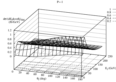
Figure 2. The standard model double differential cross-section as in figure 1, but for beam polarizations P_{e^-} = -P_{e^+} = -1 . The bottom plane shows a few contours of constant cross-section.
