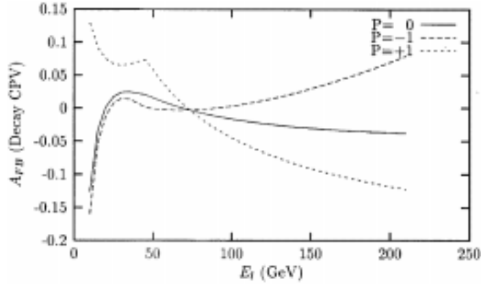
Figure 15. The asymmetry A_{FB} arising from the CP-violating tbW vertex as a function of E_l for \theta_0 = 30^\circ for three values of the effective e^+e^- polarization P . \text{Re}f_{2R} = -\text{Re}\bar{f}_{2L} = 0.1 is assumed.
