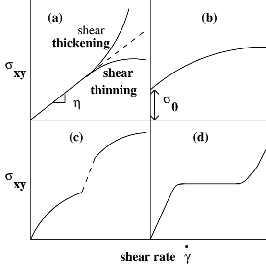
Figure 3. (a) shows Newtonian ( \sigma_{xy} = \eta\dot{\gamma}_0 ), shear thinning and shear thickening behaviours seen in viscoelastic fluids. (b) shows the flow curve of a Herschel–Bulkley plastic with a finite yield stress \sigma_0 . At \sigma_{xy} < \sigma_0 , the material behaves like a solid. At \sigma_{xy} > \sigma_0 , \sigma_{xy} = \sigma_0 + K_p\dot{\gamma}^p , which reduces to the Bingham equation for p = 1 . (c) shows the flow curve of a system undergoing a flow-induced phase transition, characterized by a sudden jump in \sigma as shown by the dotted line. (d) shows a flow curve showing a plateau region, which is a signature of shear banding.
