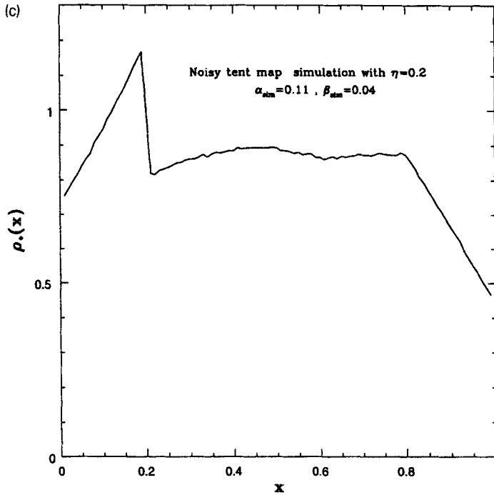
Figure 3. Numerical solution and comparison with simulation for the invariant density \rho(x) = \alpha\delta(x) + \beta\delta(1-x) + \rho_*(x) of the noisy tent map with noise amplitude \eta = 0.2 . (a) Solution after 2 iterations, starting with the zeroth approximation \rho_*(x) = 1 . The solution essentially stabilizes (correct to 3 decimal places) in 3 iterations. (b) Solution after 10 iterations. (c) The result of a numerical simulation on the noisy tent map with the re-injection prescription, (4.2). The result shown is an average over 10 simulations of 10^6 iterations each, with a bin size of 10^{-2} .
