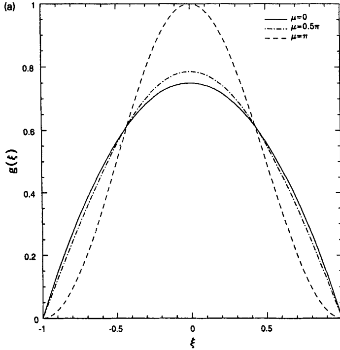
Figure 2(a). The noise distribution g(\xi; \mu) of (3.25) in the limiting cases \mu = \pi (3.27) and \mu = 0 (3.29). Also shown is the case \mu = \pi/2 , i.e., g(\xi; \pi/2) = (\pi/4) \cos(\pi\xi/2) .
