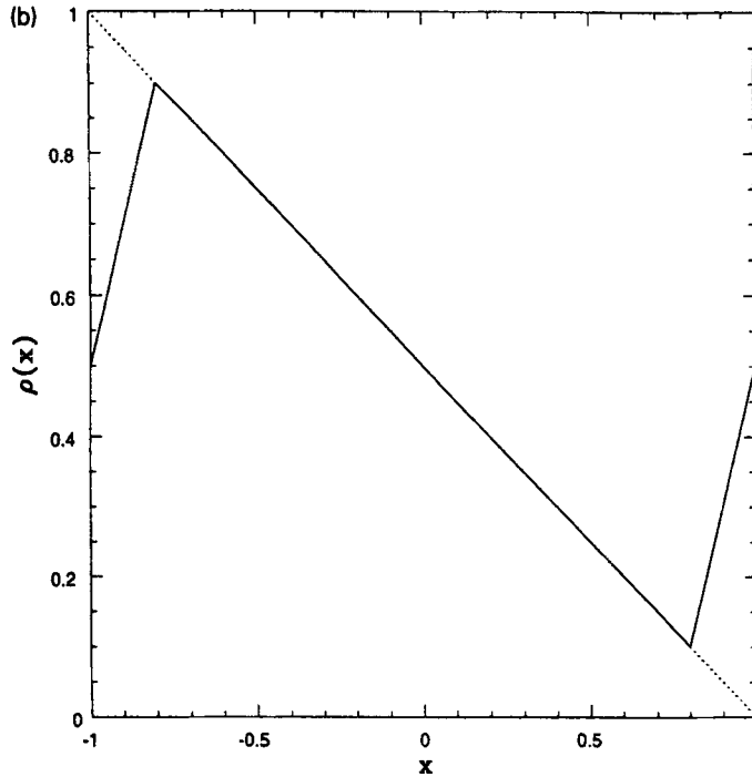
Figure 1(b). The invariant density \rho(x) for the symmetric cusp map f(x) = 1 - 2|x|^{1/2} in the presence of additive noise distributed as in figure 1(a), under periodic boundary conditions. The dotted line depicts the invariant density (1 - x)/2 of the unperturbed (noise-free) map.
