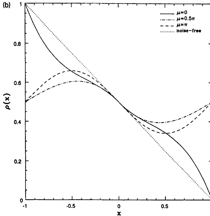
Figure 2(b). The corresponding invariant densities (3.26) for the noisy, symmetric cusp map, given by (3.28) for \mu = \pi and by (3.30) for \mu = 0 . Also shown is the case \mu = \pi/2 , for which \rho(x) = \frac{1}{2}(2 - x - \cos(\pi x/2)) ( x > 0 ) and \rho(x) = \frac{1}{2}(\cos(\pi x/2) - x) ( x < 0 ).
