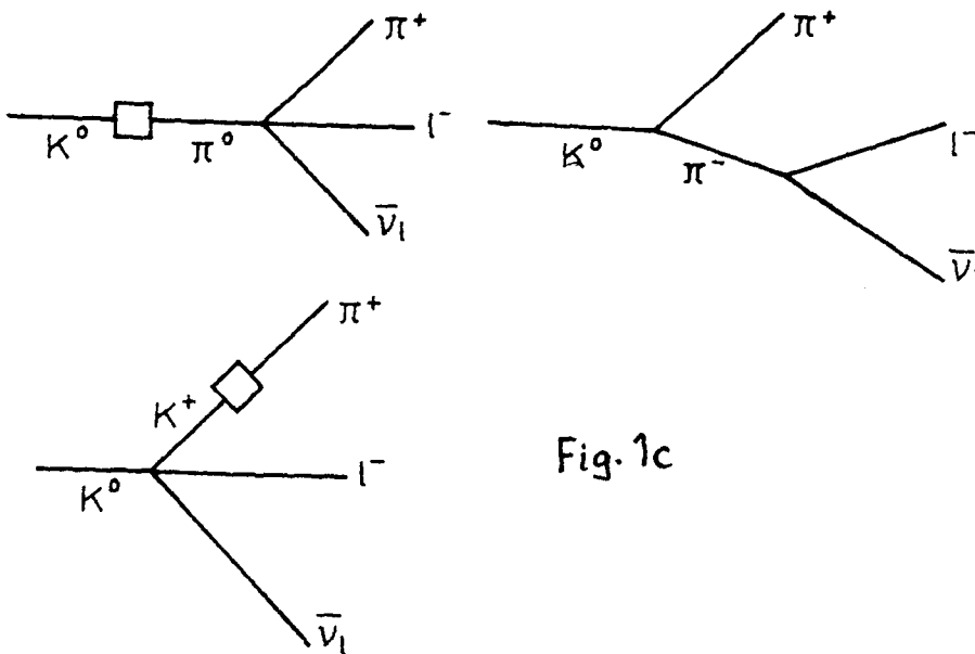
Figure 1. Diagrams relevant for the decays (a) K^0 \rightarrow K^+ e^- \bar{\nu}_e , (b) K^+ \rightarrow \gamma \gamma e^+ \nu_e , (c) \Delta S = -\Delta Q decays K^0 \rightarrow \pi^+ l^- \bar{\nu}_l .
