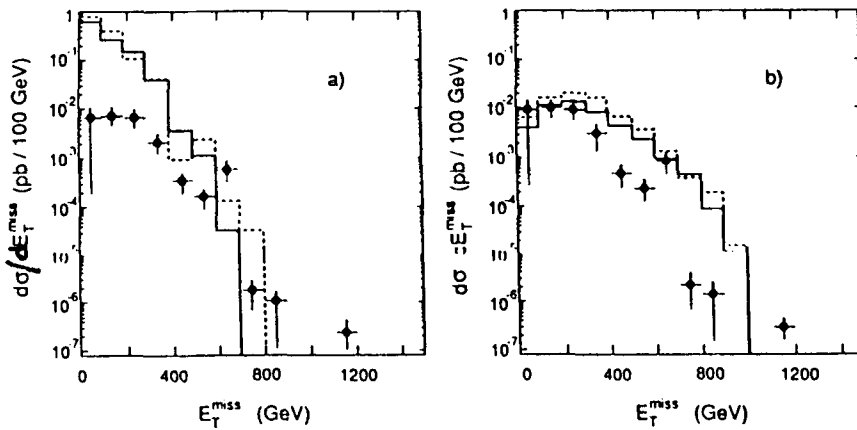
Figure 14. ISA JET Monte Carlo prediction for missing -E_T distribution after selection cuts for (a) M_{\tilde{g}} = 300 \text{ GeV} and (b) m_{\tilde{g}} = 100 \text{ GeV} at LHC. The solid (dashed) line corresponds to the gluino signal for \tan \beta = 2(10) , while the points represent the total SM background [25].
