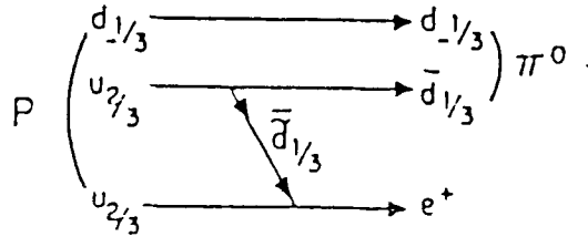
Figure 10. The proton decay process arising from squark exchange.
