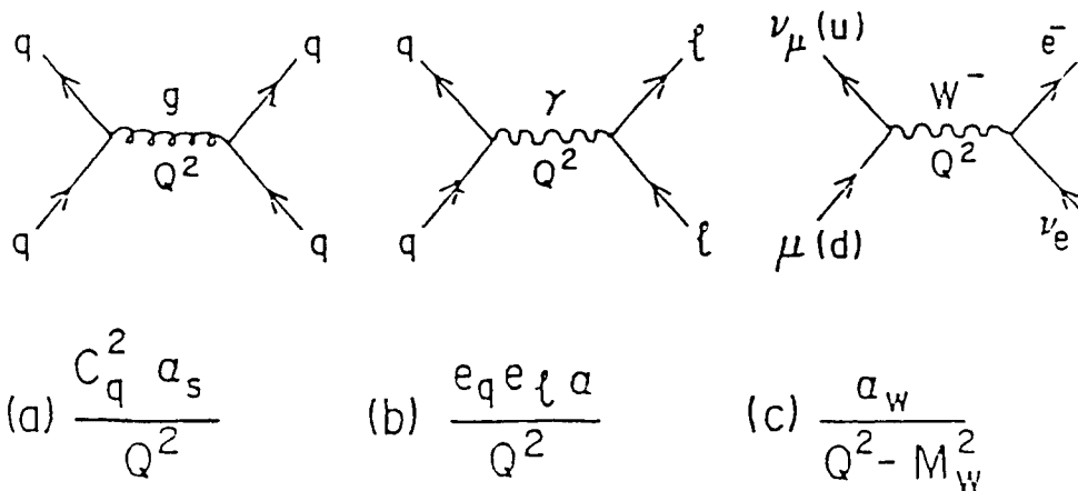
Figure 1. The basic amplitudes of (a) strong, (b) electromagnetic and (c) charged current weak interaction.
