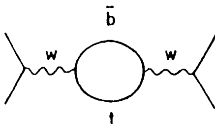
Figure 3. Radiative correction to the W boson mass arising from the t\bar{t} loop.
