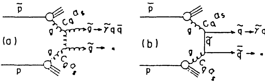
Figure 13. Pair production of (a) gluino and (b) squark via gluon-gluon fusion.
