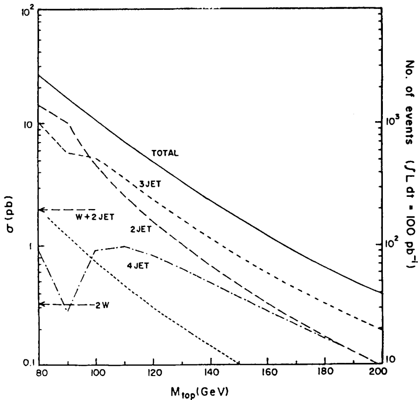
Figure 5. Top quark contribution to the isolated lepton plus n -jet events and also dilepton events (dotted line) shown for the typical energy (2 TeV) and luminosity ( 100 \text{ pb}^{-1} ) of the Tevatron upgrade. The background to the 2-jet events from W plus 2-jet and W pair production processes are also shown [12].
