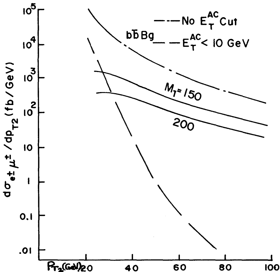
Figure 8. The expected t\bar{t} signal at LHC in the cleanest ( e\mu ) channel shown against the p_T of the 2nd (softer) lepton. The b\bar{b} background with and without the isolation cut are also shown [14].
