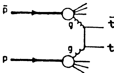
Figure 4. Top quark production in \bar{p}p ( pp ) collision via gluon-gluon fusion.
