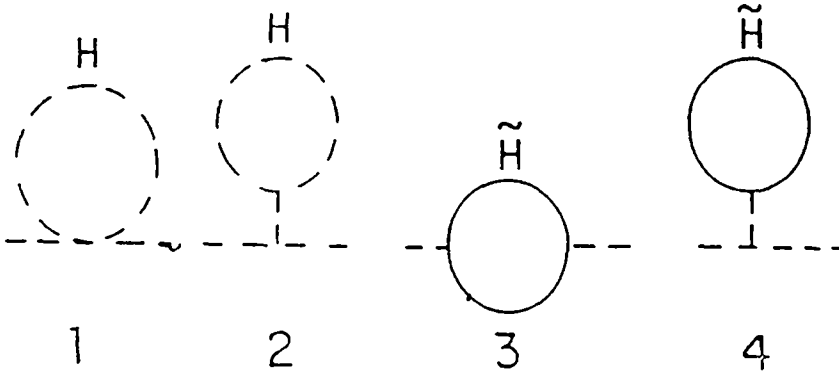
Figure 2. The quadratically divergent contributions to the Higgs mass from the radiative Higgs loops (1,2) and the cancelling SUSY contribution from the Higgsino loops (3,4).
