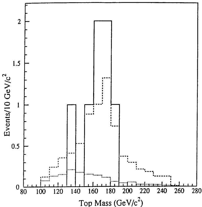
Figure 7. Top mass distribution for the data (solid histogram) and the background of 1.4 W + \text{multijets} Monte Carlo events (dots) having a tagged b . The dashed histogram represents the sum of 5.6 t\bar{t} Monte Carlo events with M_t = 175 GeV plus the 1.4 background events [2].
