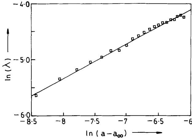
Figure 2. A typical log-log plot of \lambda vs (a - a_\infty) for z = 1.2 . The slope of the line gives the scaling exponent \nu .
