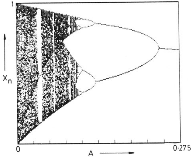
Figure 4. Bifurcation structure of the map in (6). With \mu = 4 and A = 0 , the system is fully chaotic. As A is slowly tuned, periodic cycles are traced in the reverse direction.
