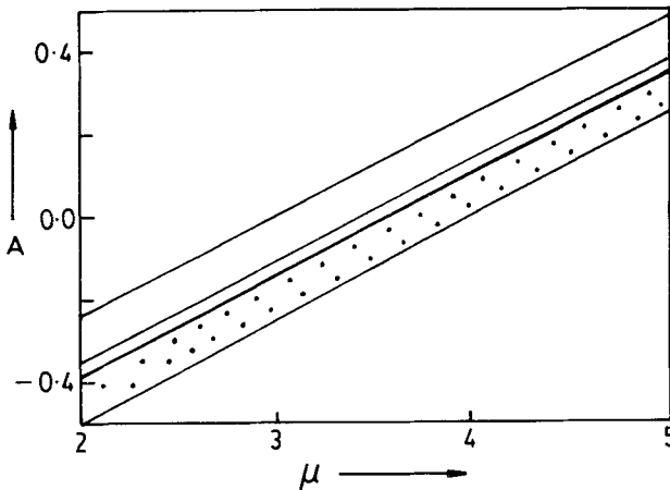
Figure 5. The parameter space (\mu, A) of the combination map. The thick line represents the transition from order to chaos while the lines parallel to it, are the bifurcation curves.
