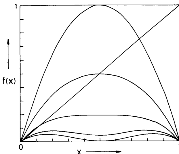
Figure 3. The combination map f(X) given in (6) for \mu = 4 . The curves correspond to A = 0, 0.5, 8/\pi^2, 3/\pi and 1 in that order from top to bottom.
