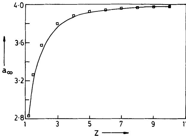
Figure 1. Variation of a_\infty with z , the order of the maximum of the map. Note that as z increases, the chaotic regime a_\infty < a < 4 shrinks and becomes very narrow for z > 10 .
